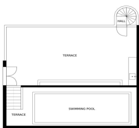
FLOOR 2
